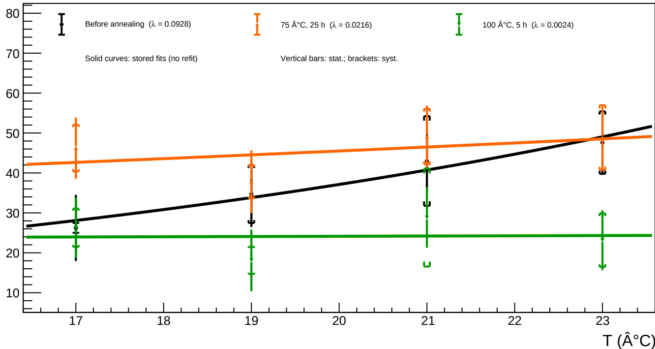
A1_v=5 - Spot 5 ( x = 231.79 , y = 755.43 ): luminosity vs temperature for all annealing phases
