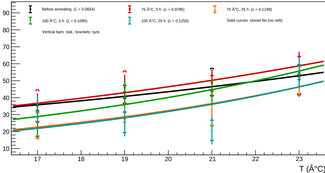
A1_v=5 - Spot 50 ( x = 1536.49 , y = 405.35 ): luminosity vs temperature for all annealing phases
