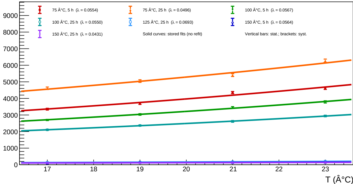
A1_v=5 - Spot 54 ( x = 1733.26 , y = 723.59 ): luminosity vs temperature for all annealing phases
