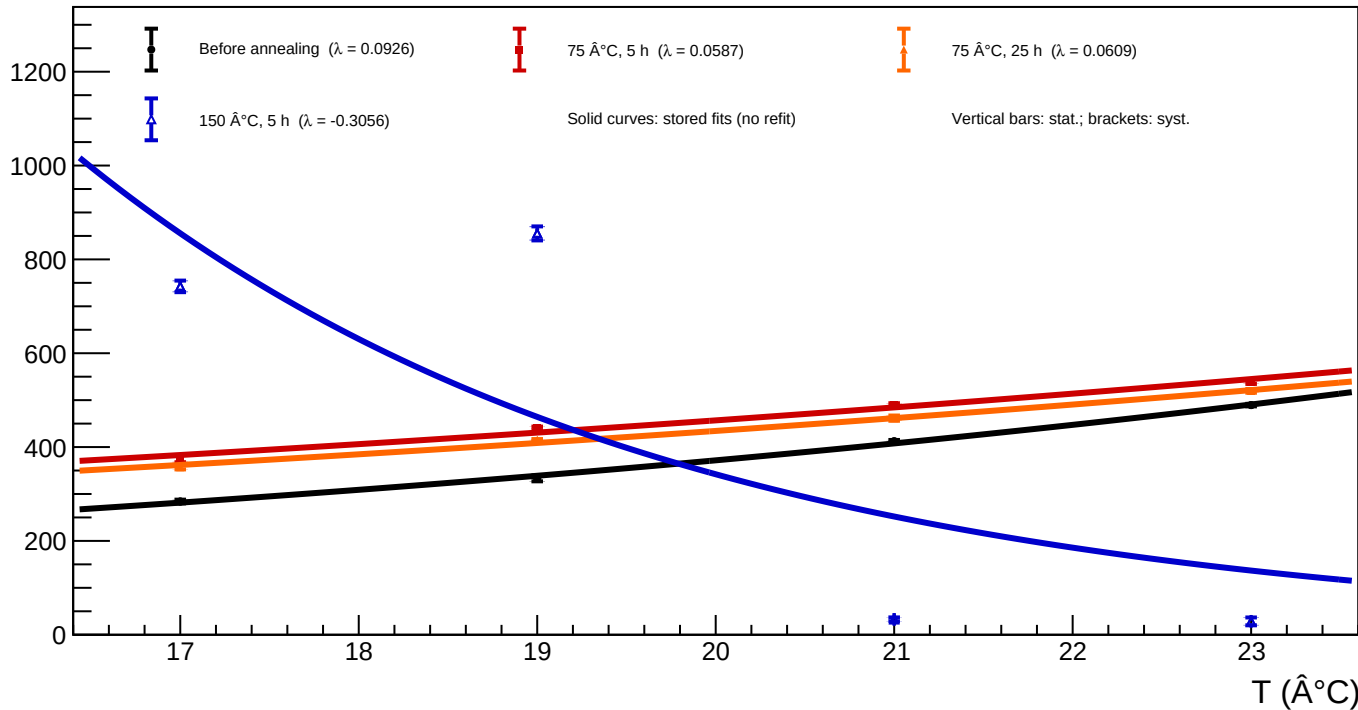
A1_v=5 - Spot 55 ( x = 1772.62 , y = 478.35 ): luminosity vs temperature for all annealing phases
