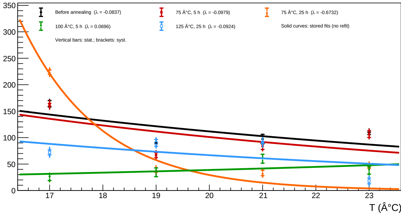
A1_v=5 - Spot 58 ( x = 1821.28 , y = 993.08 ): luminosity vs temperature for all annealing phases
