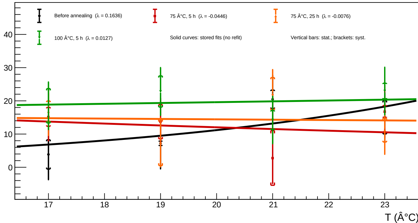
A1_v=5 - Spot 60 ( x = 1655.35 , y = 493.99 ): luminosity vs temperature for all annealing phases
