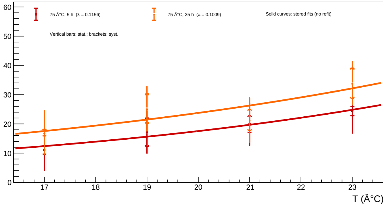
A1_v=5 - Spot 63 (x = 899.84, y = 255.46): luminosity vs temperature for all annealing phases
