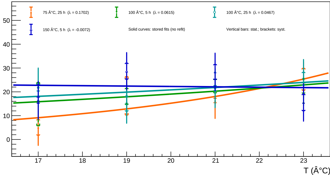
A1_v=5 - Spot 68 (x = 262.26, y = 494.00): luminosity vs temperature for all annealing phases
