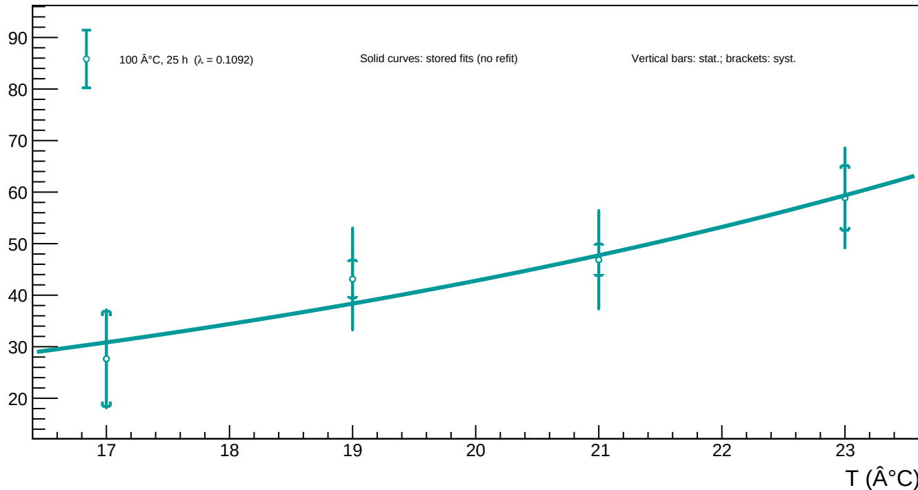
A1_v=5 - Spot 69 (x = 93.94, y = 351.54): luminosity vs temperature for all annealing phases
