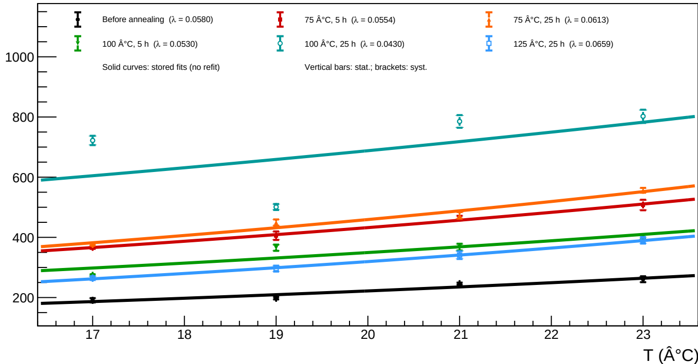
A1_v=5 - Spot 7 (x = 253.82, y = 349.89): luminosity vs temperature for all annealing phases
