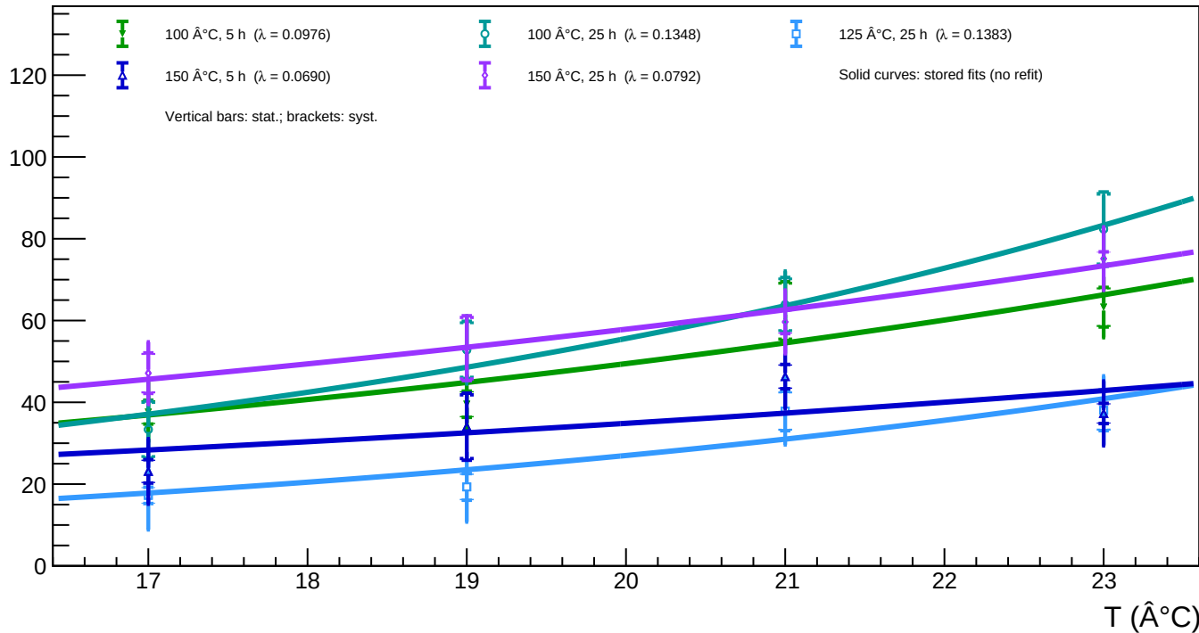
A1_v=5 - Spot 70 ( x = 337.15 , y = 286.11 ): luminosity vs temperature for all annealing phases
