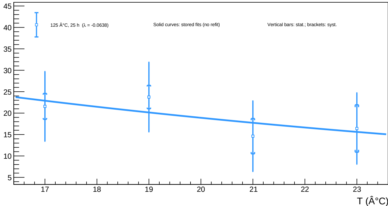
A1_v=5 - Spot 84 ( x = 1807.84 , y = 451.97 ): luminosity vs temperature for all annealing phases
