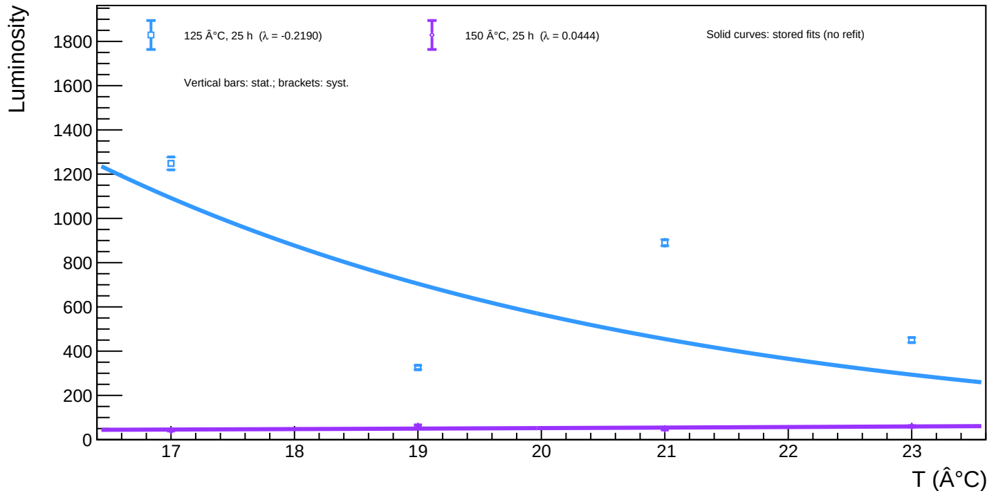
A1_v=5 - Spot 85 (x = 830.57, y = 884.46): luminosity vs temperature for all annealing phases
