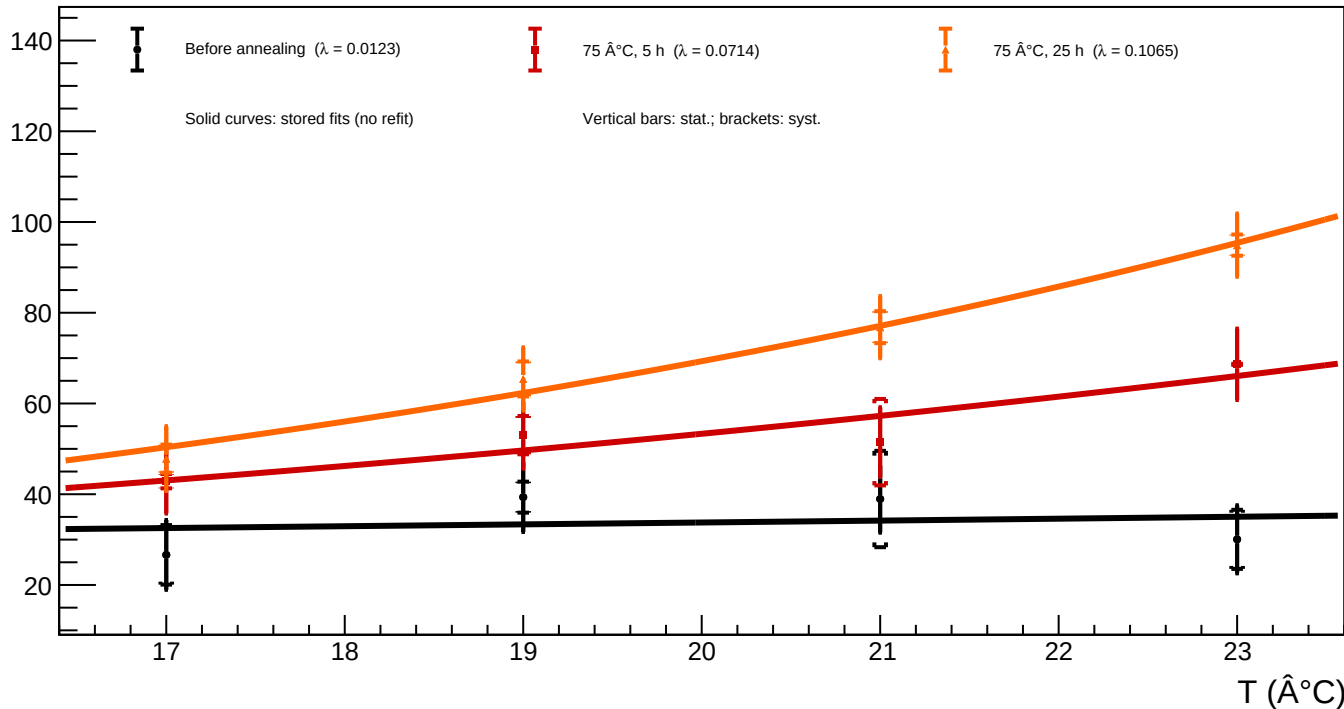
A1_v=5 - Spot 9 ( x = 375.21 , y = 368.35 ): luminosity vs temperature for all annealing phases
