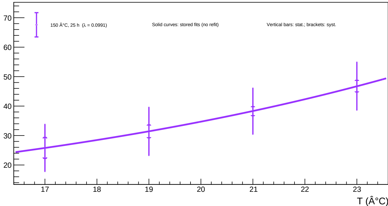
A1_v=5 - Spot 95 (x = 806.54, y = 192.06): luminosity vs temperature for all annealing phases
