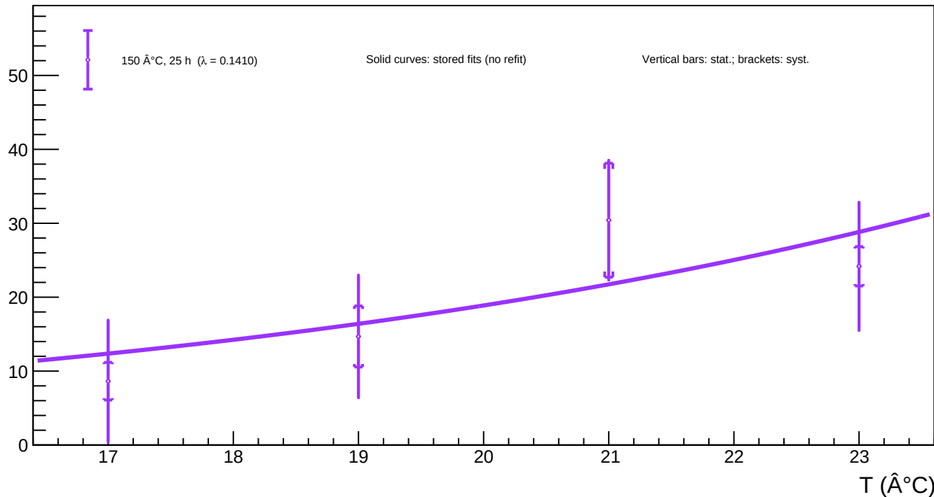
A1_v=5 - Spot 97 ( x = 1733.48 , y = 123.65 ): luminosity vs temperature for all annealing phases
