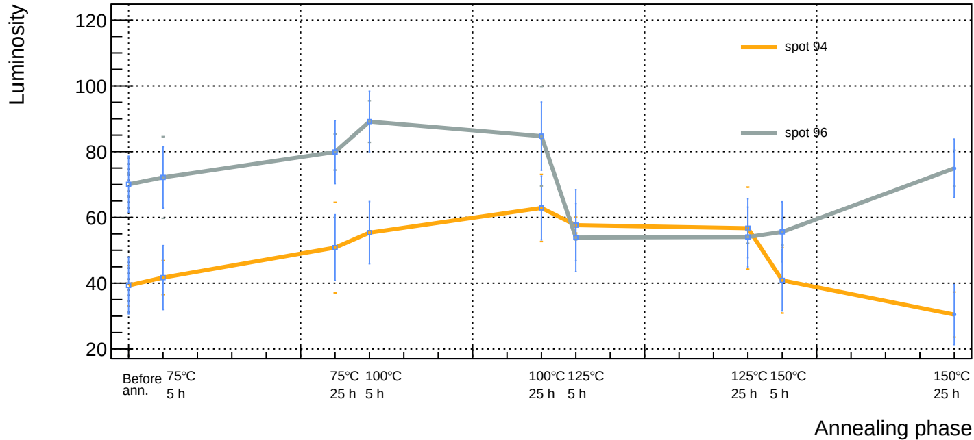
Sensor A1, T = 20\text{ }^{\circ}\text{C} , v_{\text{over}} = 7\text{ V} - Approximately constant hotspots
