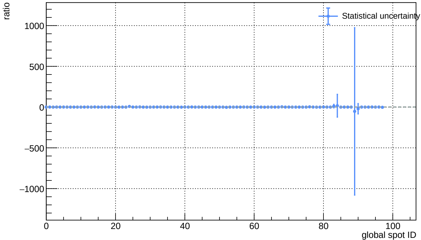
Sensor A1, T = 20 C - L(\text{ann\_150C\_5h}) / L(\text{before\_annealing})
