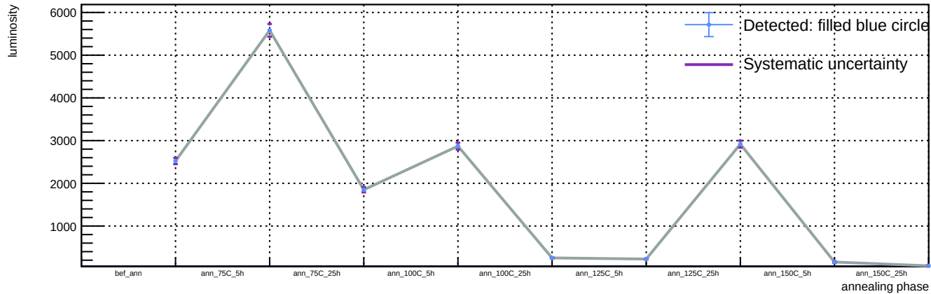
Sensor A1, T = 20\text{ C} , v_{\text{over}} = 7\text{ V} - Spot 0: luminosity vs phase
