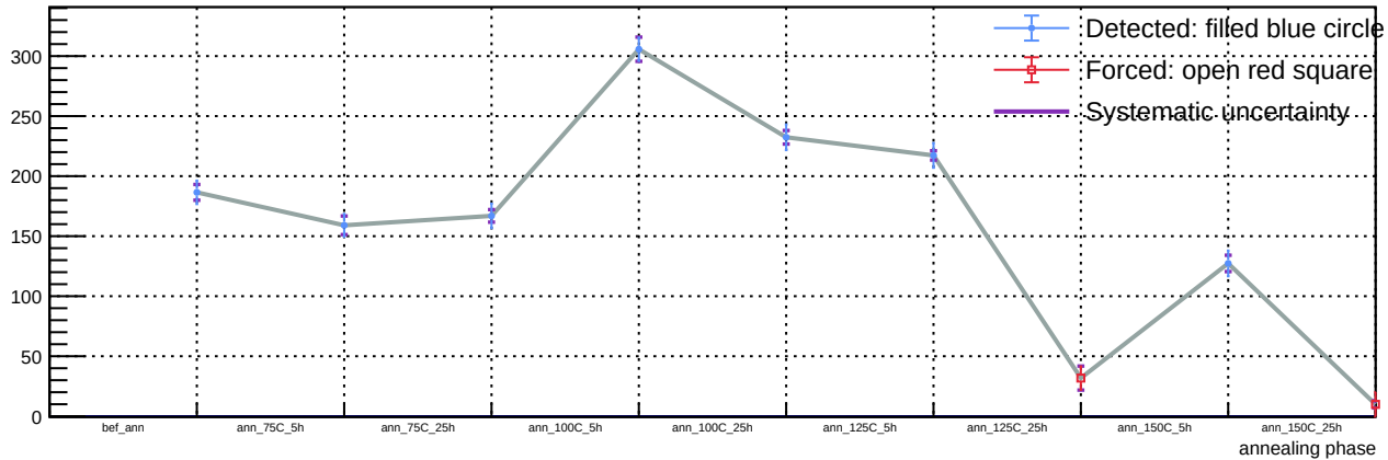
Sensor A1, T = 20\text{ C} , v_{\text{over}} = 7\text{ V} - Spot 1: luminosity vs phase
