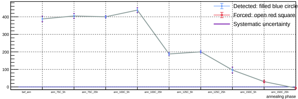
Sensor A1, T = 20\text{ C} , v_{\text{over}} = 7\text{ V} - Spot 10: luminosity vs phase
