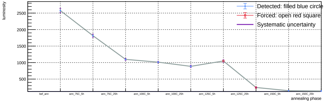
Sensor A1, T = 20\text{ C} , v_{\text{over}} = 7\text{ V} - Spot 13: luminosity vs phase
