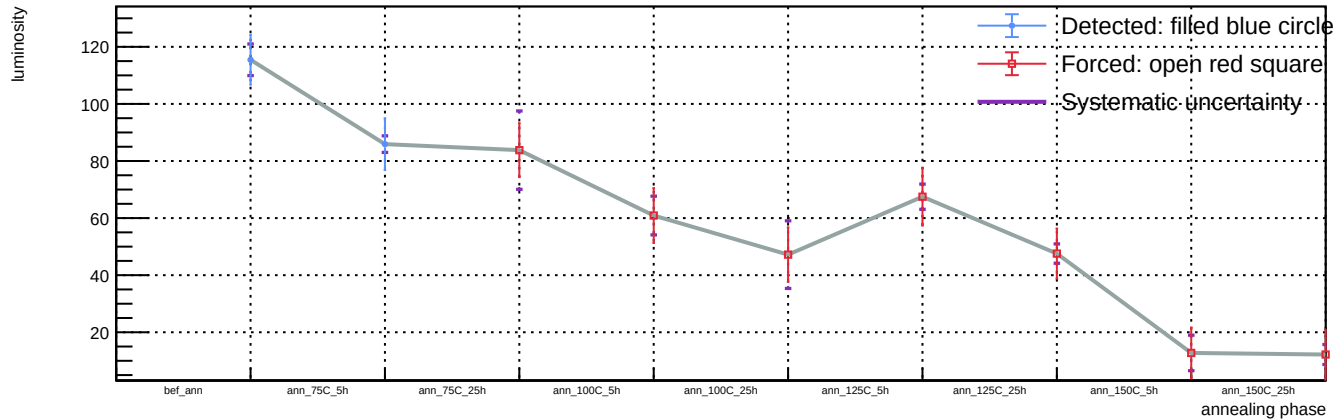
Sensor A1, T = 20\text{ C} , v_{\text{over}} = 7\text{ V} - Spot 15: luminosity vs phase
