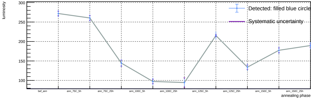
Sensor A1, T = 20\text{ C} , v_{\text{over}} = 7\text{ V} - Spot 17: luminosity vs phase
