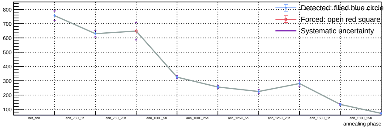
Sensor A1, T = 20\text{ C} , v_{\text{over}} = 7\text{ V} - Spot 22: luminosity vs phase
