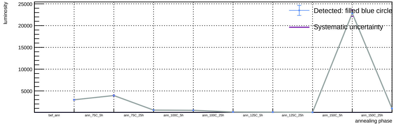
Sensor A1, T = 20\text{ C} , v_{\text{over}} = 7\text{ V} - Spot 24: luminosity vs phase
