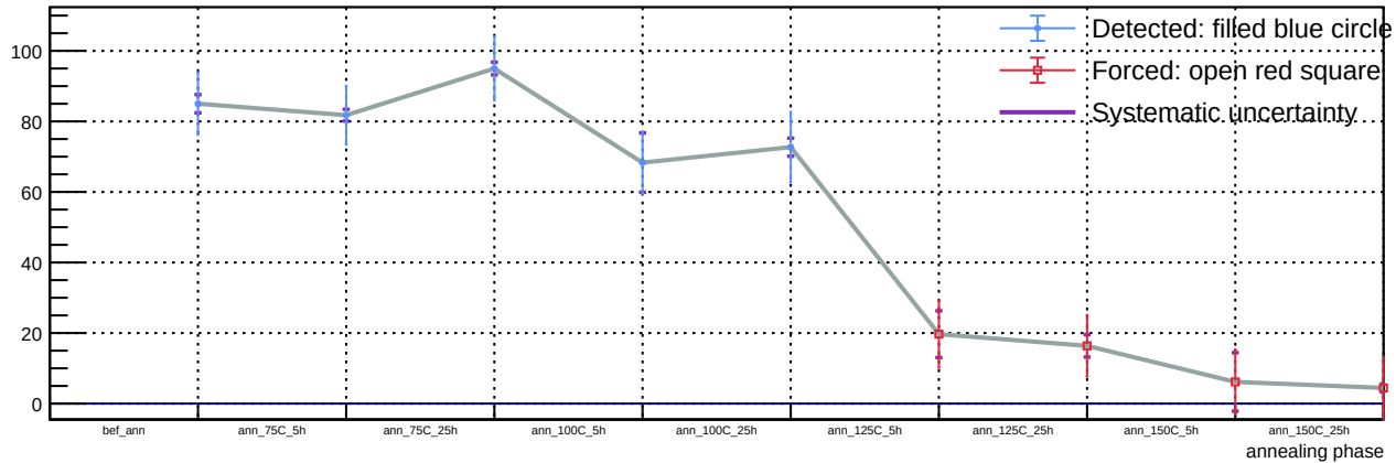
Sensor A1, T = 20\text{ C} , v_{\text{over}} = 7\text{ V} - Spot 26: luminosity vs phase
