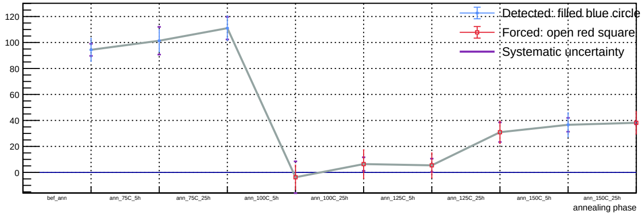
Sensor A1, T = 20\text{ C} , v_{\text{over}} = 7\text{ V} - Spot 34: luminosity vs phase
