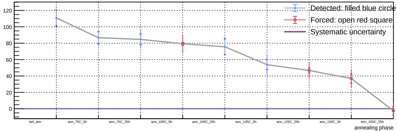
Sensor A1, T = 20\text{ C} , v_{\text{over}} = 7\text{ V} - Spot 36: luminosity vs phase
