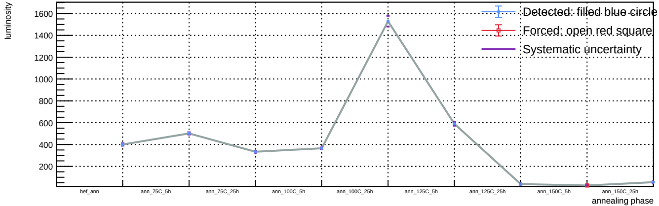
Sensor A1, T = 20\text{ C} , v_{\text{over}} = 7\text{ V} - Spot 37: luminosity vs phase
