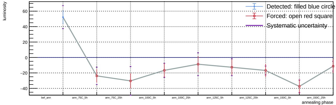
Sensor A1, T = 20\text{ C} , v_{\text{over}} = 7\text{ V} - Spot 39: luminosity vs phase
