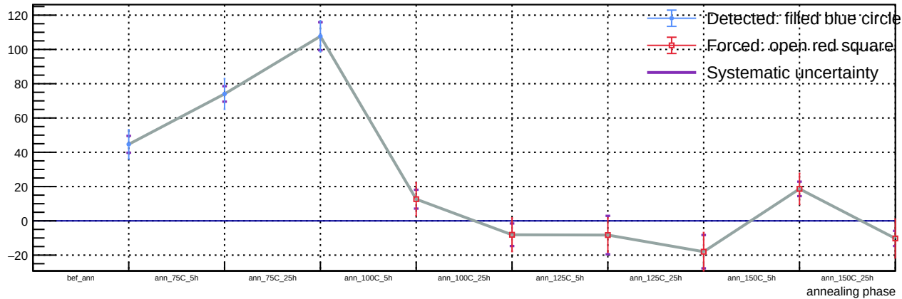
Sensor A1, T = 20\text{ C} , v_{\text{over}} = 7\text{ V} - Spot 44: luminosity vs phase
