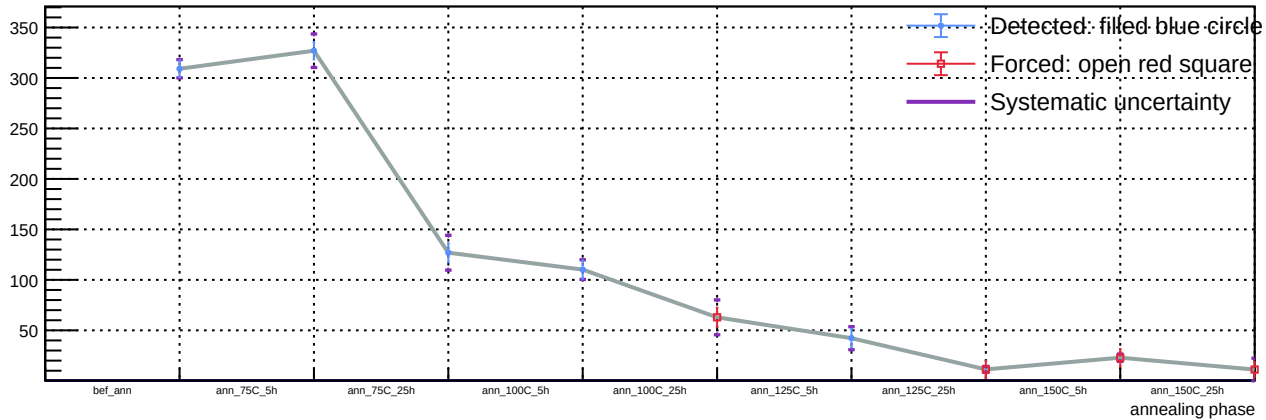
Sensor A1, T = 20\text{ C} , v_{\text{over}} = 7\text{ V} - Spot 49: luminosity vs phase
