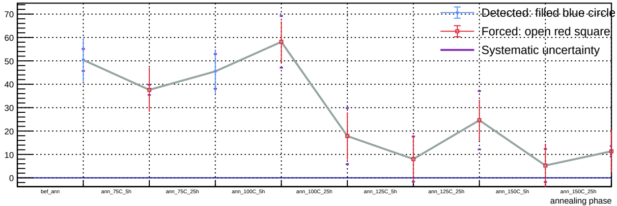
Sensor A1, T = 20\text{ C} , v_{\text{over}} = 7\text{ V} - Spot 51: luminosity vs phase
