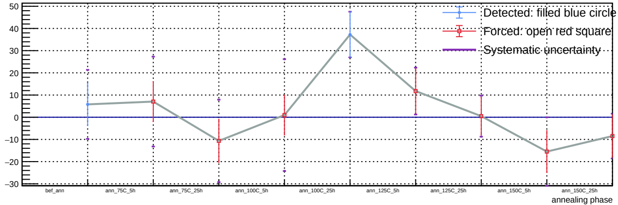
Sensor A1, T = 20\text{ C} , v_{\text{over}} = 7\text{ V} - Spot 52: luminosity vs phase
