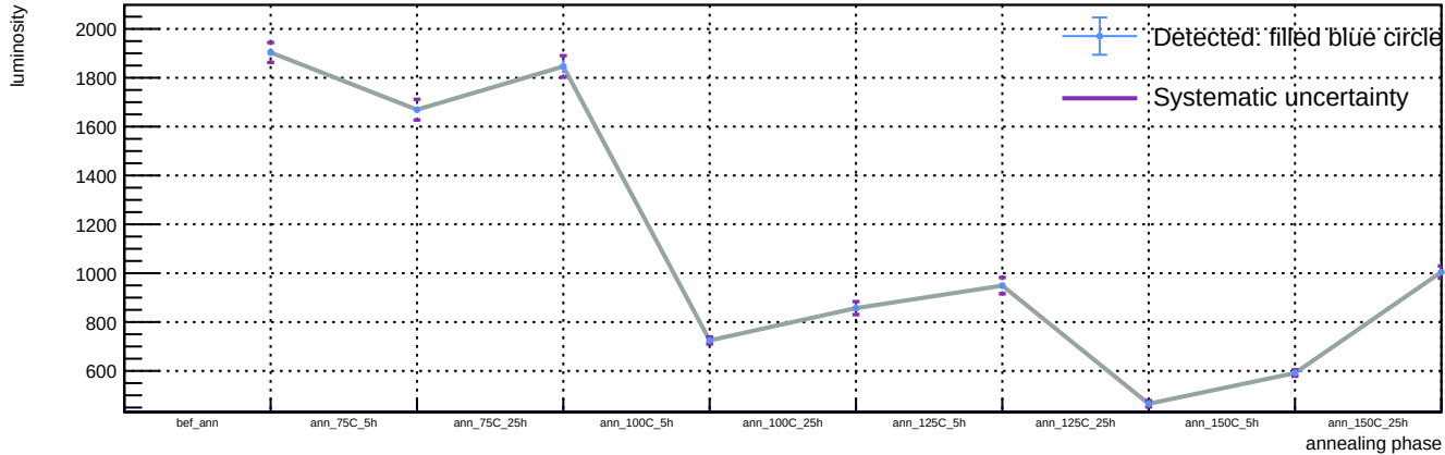
Sensor A1, T = 20\text{ C} , v_{\text{over}} = 7\text{ V} - Spot 6: luminosity vs phase
