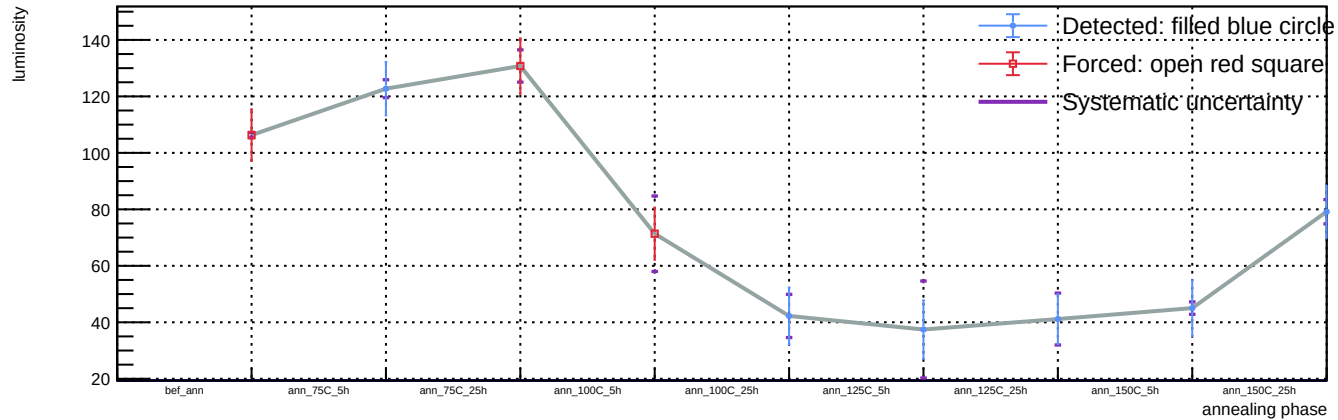
Sensor A1, T = 20\text{ C} , v_{\text{over}} = 7\text{ V} - Spot 61: luminosity vs phase
