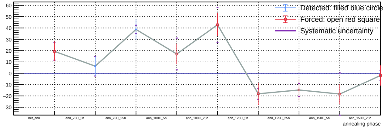
Sensor A1, T = 20\text{ C} , v_{\text{over}} = 7\text{ V} - Spot 63: luminosity vs phase
