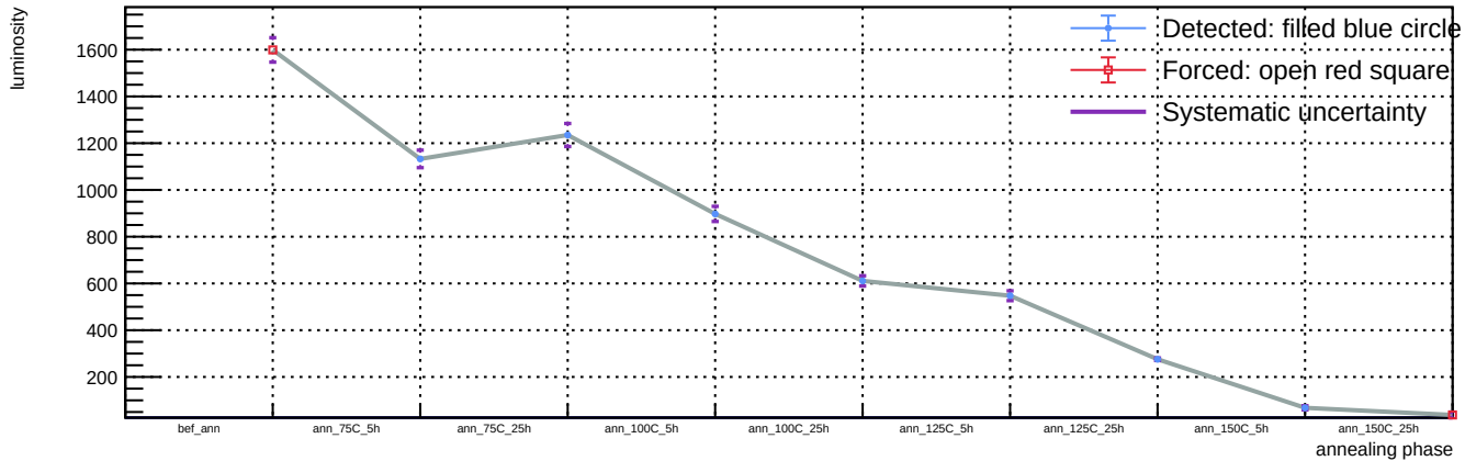
Sensor A1, T = 20\text{ C} , v_{\text{over}} = 7\text{ V} - Spot 64: luminosity vs phase
