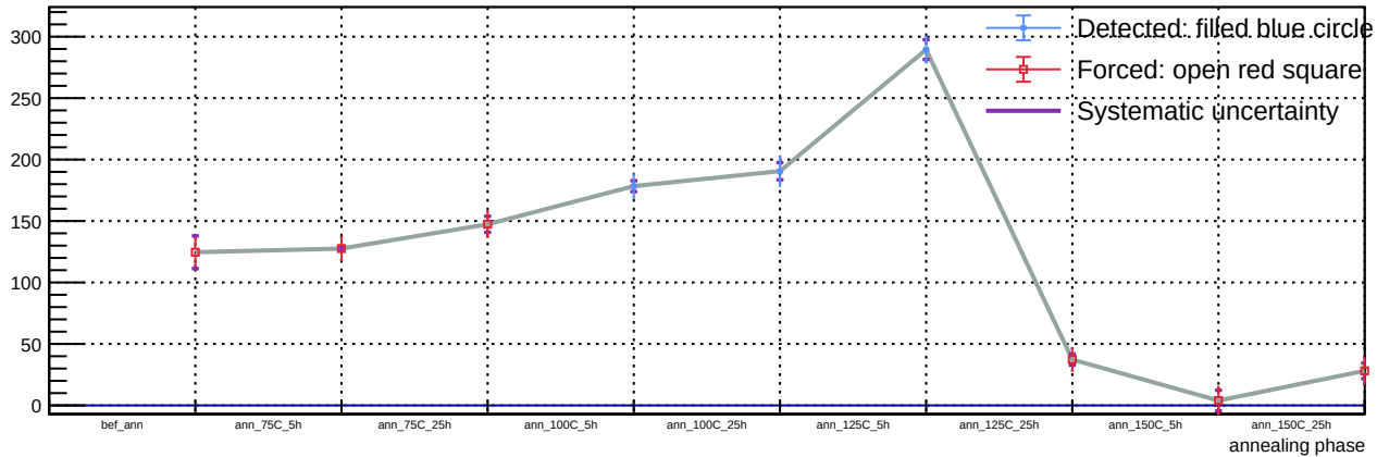
Sensor A1, T = 20\text{ C} , v_{\text{over}} = 7\text{ V} - Spot 71: luminosity vs phase
