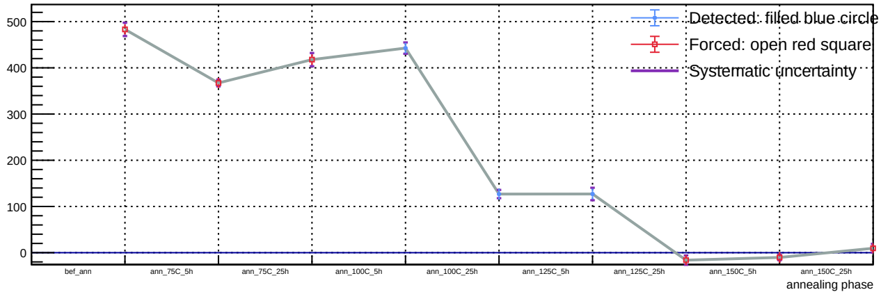
Sensor A1, T = 20\text{ C} , v_{\text{over}} = 7\text{ V} - Spot 72: luminosity vs phase
