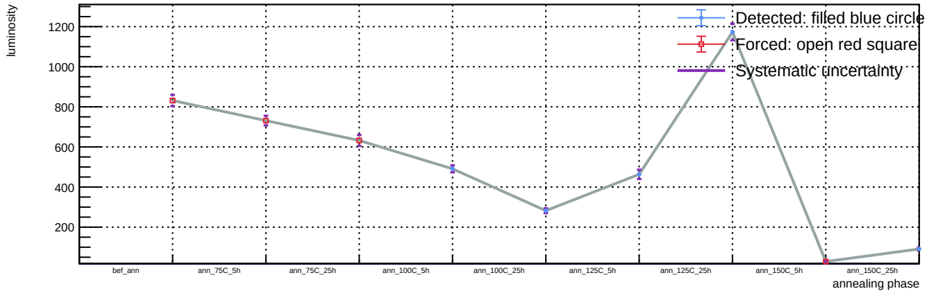
Sensor A1, T = 20\text{ C} , v_{\text{over}} = 7\text{ V} - Spot 73: luminosity vs phase
