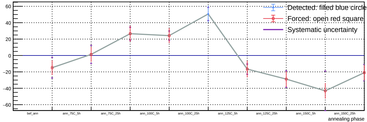
Sensor A1, T = 20\text{ C} , v_{\text{over}} = 7\text{ V} - Spot 76: luminosity vs phase
