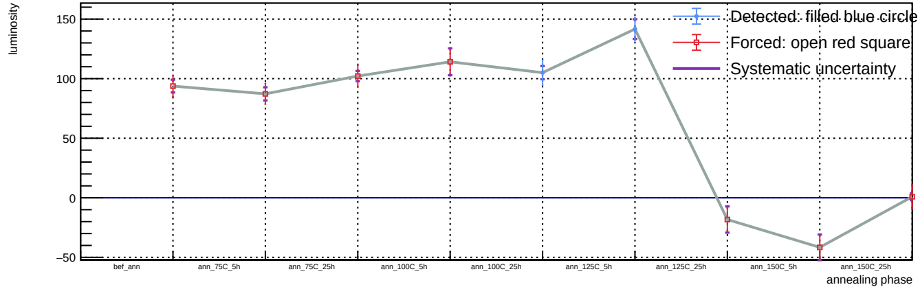
Sensor A1, T = 20\text{ C} , v_{\text{over}} = 7\text{ V} - Spot 79: luminosity vs phase
