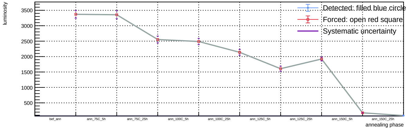
Sensor A1, T = 20\text{ C} , v_{\text{over}} = 7\text{ V} - Spot 85: luminosity vs phase
