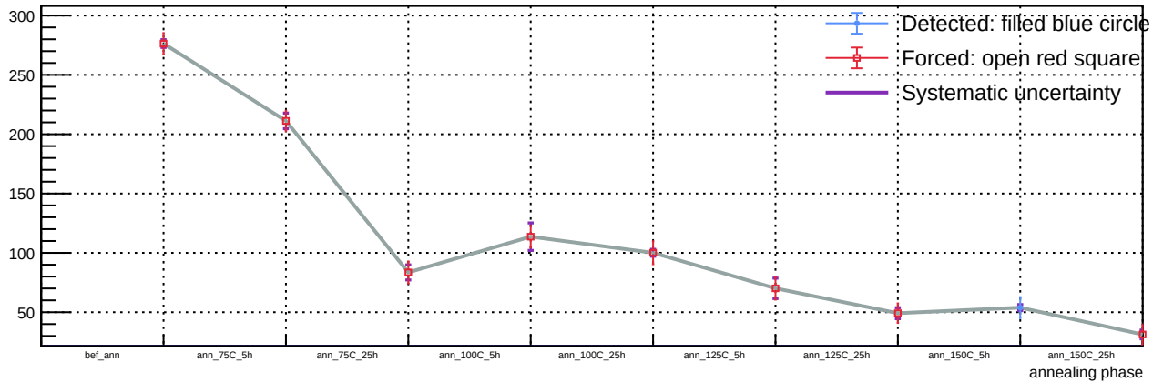
Sensor A1, T = 20\text{ C} , v_{\text{over}} = 7\text{ V} - Spot 86: luminosity vs phase
