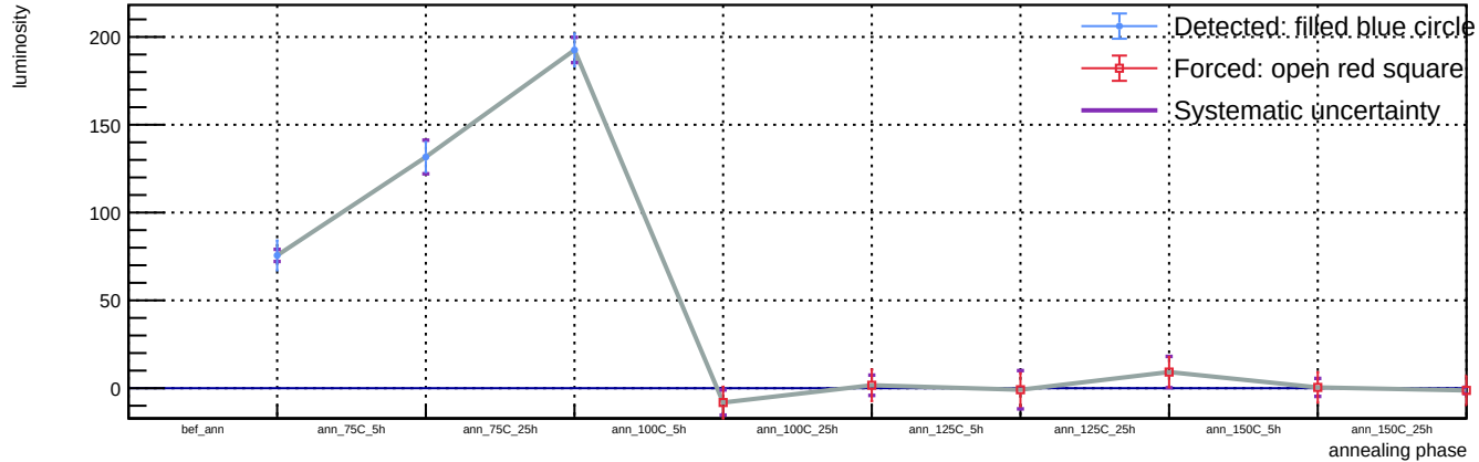
Sensor A1, T = 20\text{ C} , v_{\text{over}} = 7\text{ V} - Spot 9: luminosity vs phase
