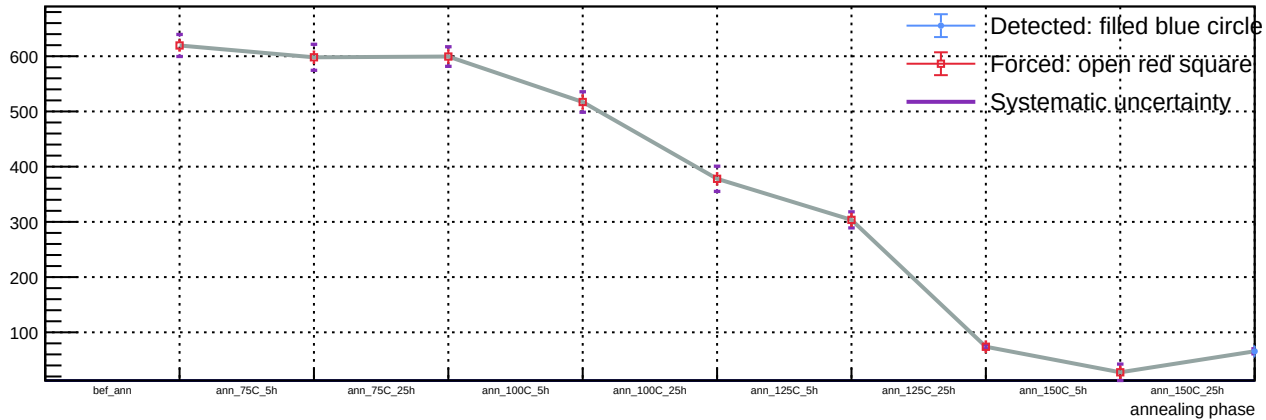
Sensor A1, T = 20\text{ C} , v_{\text{over}} = 7\text{ V} - Spot 95: luminosity vs phase
