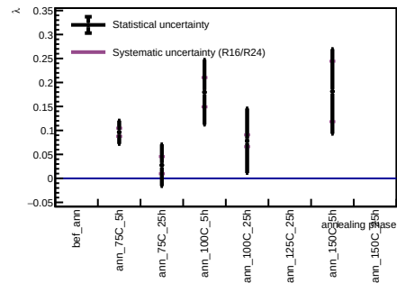
Sensor A1, v = 5 V - Spot 65
