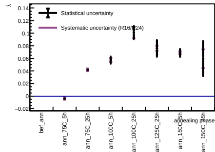
Sensor A1, v = 5 V - Spot 62
