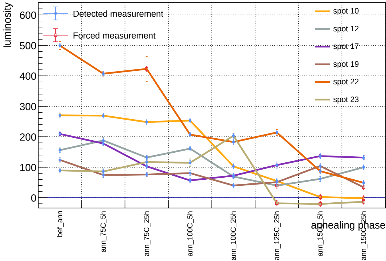
Sensor A1, v = 5 V, representative T = 23 C (max available) - luminosity vs phase - order 10^2
